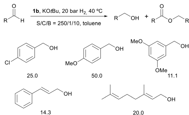
Scheme 3 Hydrogenation of aldehydes using complex 1b. All reactions proceeded with full conversion. For aryl aldehydes the numerical values correspond to the alcohol/ester ratio. In the case of cinnamaldehyde and geranial, the values indicate the ratio between the allyl alcohol and the fully hydrogenated product.
