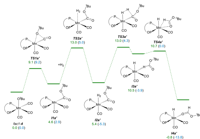
Fig. 10 General scheme for the activation of fac1-4a by Or Bu migration. Numerical values correspond to relative free (green) and electronic energies (blue, in parentheses) in kcal mol -1 relative to fac1-4 .
