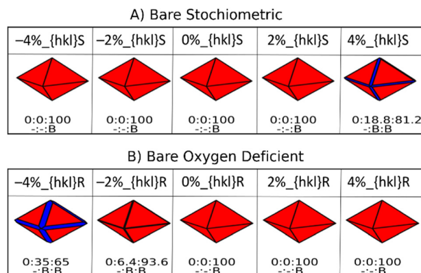
Fig. 4 The shape of \text{CeO}_2 unstrained and strained bare nanoparticles. Red, blue and green represent the \{111\} , \{110\} and \{100\} \text{CeO}_2 surfaces, respectively. The shapes of the nanoparticles are generated at a hydrogen peroxide partial pressure of 1 bar and 298 K using the Wulff construction routines in Pymatgen. 101 Each shape is characterized by a ratio of surfaces defined in numerical percentage ( \{100\}:\{110\}:\{111\} ). The label B defines a bare surface. The shape of the stoichiometric nanoparticles is redrawn from our previous work. 40
