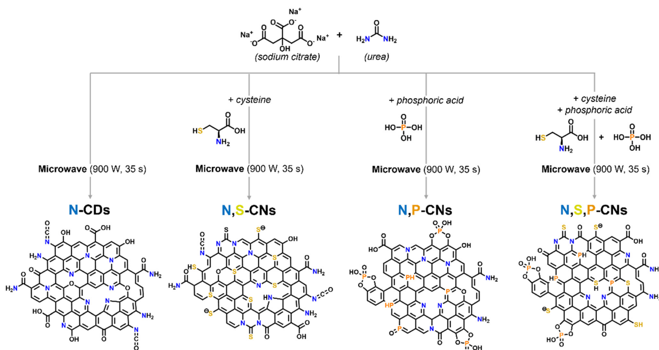
Scheme 1 Methodology for the synthesis of the multi-doped carbon nanomaterials: N-CDs; N,S-CNs; N,P-CNs; and N,S,P-CN.
