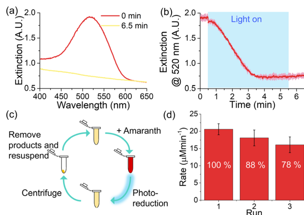
Fig. 3 (a) Extinction spectra of 0.5 mg mL -1 Flap Mix and 50 μM amaranth before and after light irradiation. (b) Extinction at 520 nm over time during the photo-reduction of amaranth with Flap Mix . (c) Scheme showing the recycling of the photocatalyst and (d) the rate of amaranth photoreduction during each sequential run ( n = 3).
