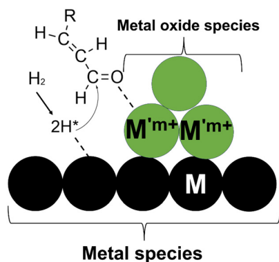
Scheme 2 Proposed reaction mechanism for unsaturated aldehyde hydrogenation and polyol hydrogenolysis over bimetallic M– \text{M}'\text{O}_x catalysts.
