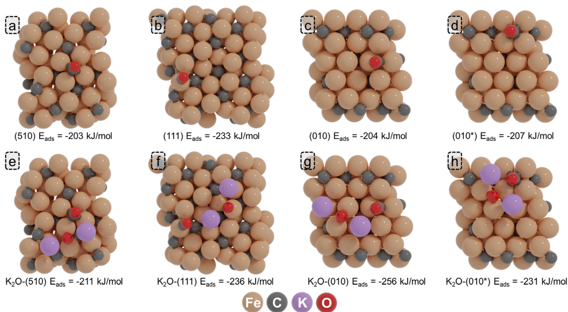
Fig. 2 The most stable adsorption structures and energy values of CO on (a–d) the pristine and (e–h) \text{K}_2\text{O} -promoted (510), (111), (010) and (010*) surfaces of \chi\text{-Fe}_5\text{C}_2 .
