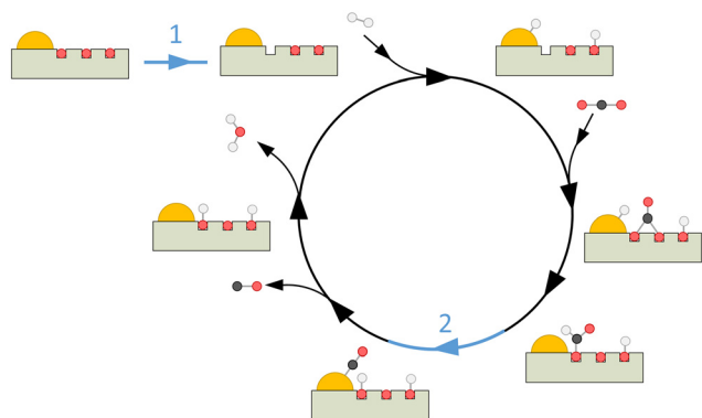
Fig. 8 Proposed associative monobridged formate-mediated reaction mechanism for the plasmonic-driven rWGS reaction over \text{Au/CeO}_{2-x} upon illumination. In fully oxidised catalysts, the rate-determining step (blue 1) is the plasmonic-driven generation of vacancies near Au NPs. For catalysts with a reducing treatment, the rate-determining step (blue 2) is proposed to be the dissociation of the formate intermediate. Atoms are labelled as Au (gold), C (black), H (white), O (red).
