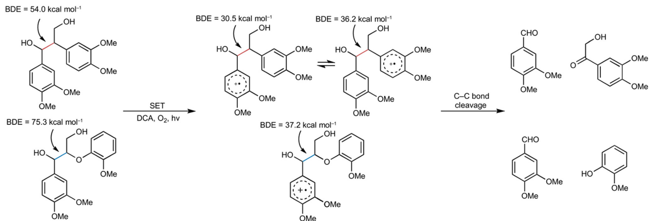
Scheme 14 C–C bond cleavage in dimeric lignin models triggered by excited 9,10-dicyanoanthracene (DCA) (this scheme has been reproduced from ref. 65 and 92 with permission from Nature Publication Group & American Chemical Society, copyright 2022 & copyright 2010).
