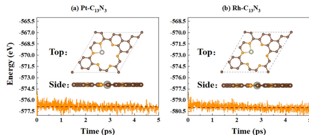
Fig. 3 Variation of energy as a function of time in the AIMD simulation within 5 ps at 1000 K for (a) Pt- \text{C}_{13}\text{N}_3 and (b) Rh- \text{C}_{13}\text{N}_3 .
