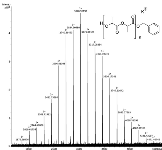
Fig. 4 MALDI-ToF-MS spectrum of PLA obtained with 20 equivalents of \text{L-LA} under reaction conditions described in run 1.
