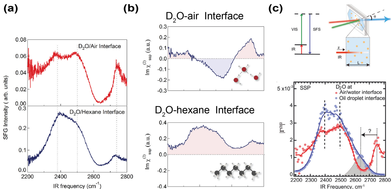
Fig. 6 Probing hydrophobic water interface using sum frequency-based spectroscopy. (a) VSGF spectrum of D 2 O–hexane and D 2 O–air interface, respectively. Reproduced with permission from ref. 129. Copyright 2015, the American Institute of Physics. (b) VSGF spectrum showing Im(χ (2) ) of D 2 O–hexane and D 2 O–air interfaces, respectively. Reproduced with permission from ref. 129. Copyright 2015, the American Institute of Physics. (c) Energy level diagram of VSFS and a schematic diagram of the experimental setup. Sum frequency scattering spectrum of D 2 O–hexadecane (blue) and water–air interface (red), respectively. Similar to the Raman-MCR spectrum, the stretching frequency of the free OD on the D 2 O–hexadecane interface is redshifted compared to the D 2 O–air interface. Reproduced with permission from ref. 132. Copyright 2021, the American Association for the Advancement of Science.
