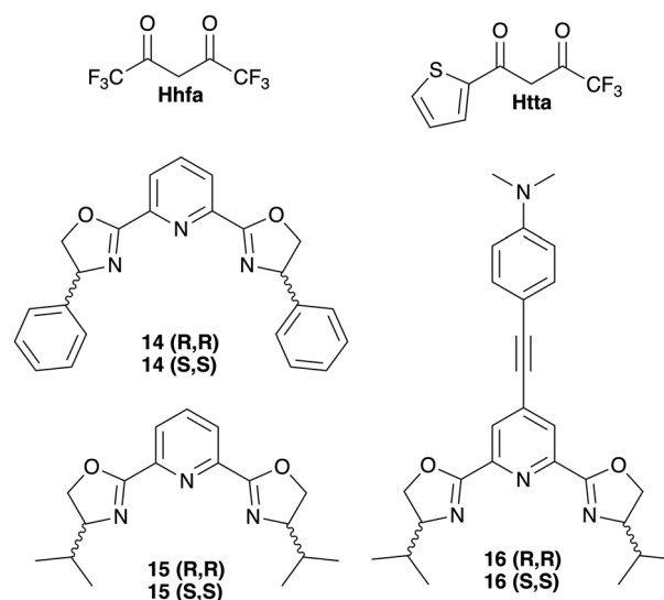
Fig. 9 Structural formulas of \beta -diketonates hexafluoroacetylacetone ( Hhfa ), 2-thenyltrifluoroacetone ( Htta ) and pyridine bis-oxazoline ( pybox )-derived chiral ligands 14–16 . 122,170
