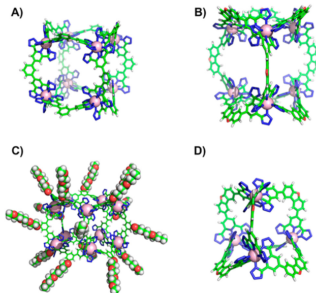
Fig. 36 Crystal structures of (A) \text{K}_{24}\text{Eu}_8(\mathbf{76})_{12} , (B) \text{K}_{18}\text{Eu}_6(\mathbf{75})_9 , and energy optimised structures of (C) \text{K}_{30}\text{Eu}_{10}(\mathbf{77})_{15} , and (D) \text{K}_{12}\text{Eu}_4(\mathbf{75})_6 . 261 Adapted from ref. 261 with permission from the American Chemical Society, Copyright©2020.
