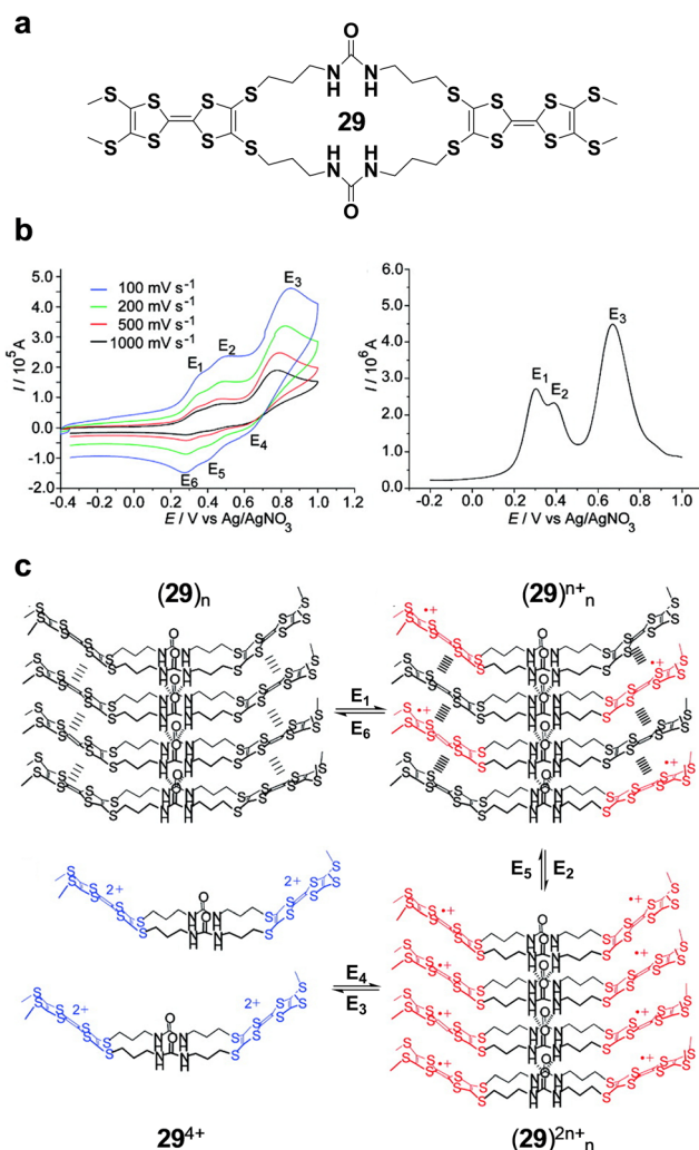
Fig. 11 (a) Chemical structure of DMTTF-containing bis-urea 29 . (b) Cyclic voltammograms of 29 ( 5 \times 10^{-5} M, DMF, \text{Ag}/\text{AgNO}_3 as reference electrode, glassy carbon as working electrode, \text{Bu}_4\text{NClO}_4 as supporting electrolyte, 298 K) at several scan rates (left) and differential pulse voltammetry of 29 under identical conditions (right). (c) Proposed redox-controlled assembly-disassembly mechanism. Adapted with permission from ref. 126. Copyright 2009-American Chemical Society.
