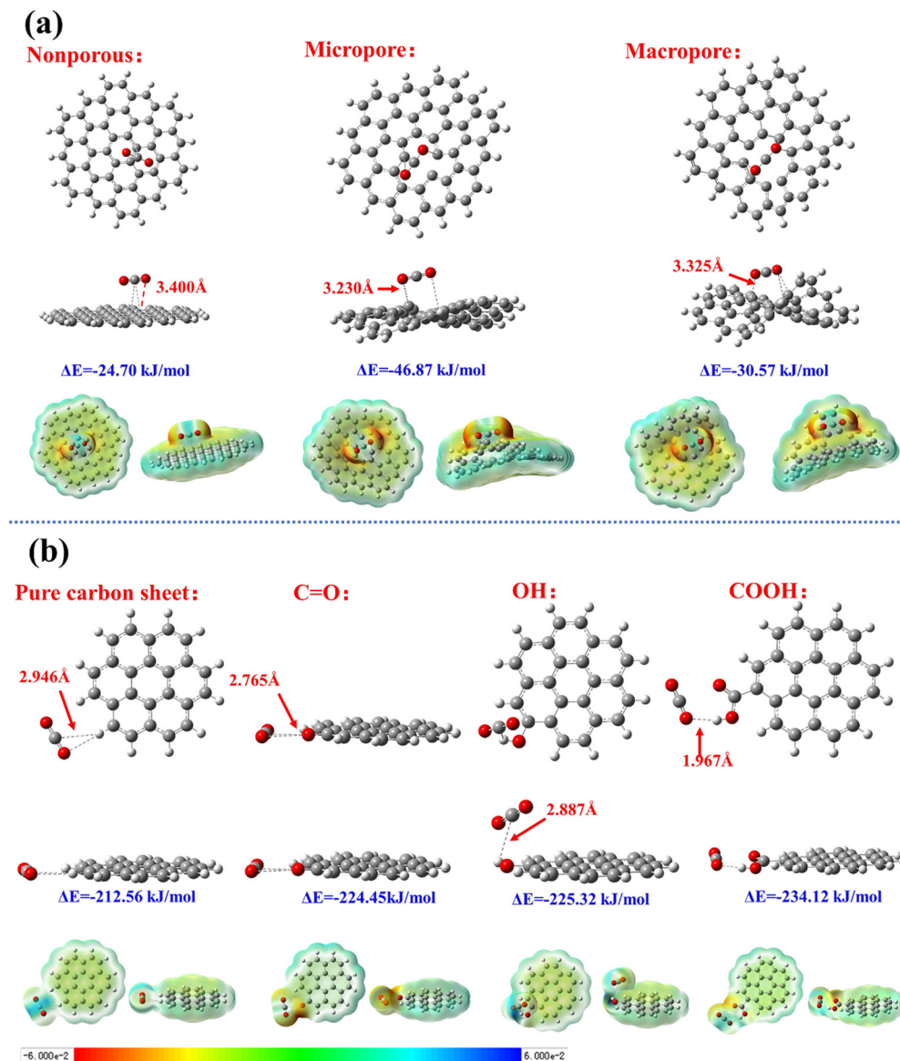
Fig. 8 Carbon sheets with varying pore sizes represented by ball-and-stick model and electron cloud density with bond lengths between the oxygen atoms of CO 2 , as well as calculated adsorption energy specified. Here, (a) depicts the comparison between interactions with different pore structures (non-porous, microporous, macroporous) and (b) shows the comparison of various functional groups on the carbon sheets (pure carbon, carbonyl, hydroxy, and carboxylic acid group). Reproduced with permission. 107 Copyright 2024, Elsevier.
