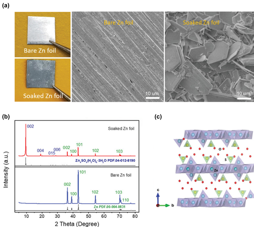
Fig. 48 (a) Photographs and SEM images and (b) XRD patterns before and after soaking Zn metal in a 1 m ZnSO_4 solution for several days. (c) Crystal structure of the byproduct, Zn_4SO_4(OH)_6 \cdot 3H_2O . 444 Reprinted with permission from Advanced Functional Materials .
