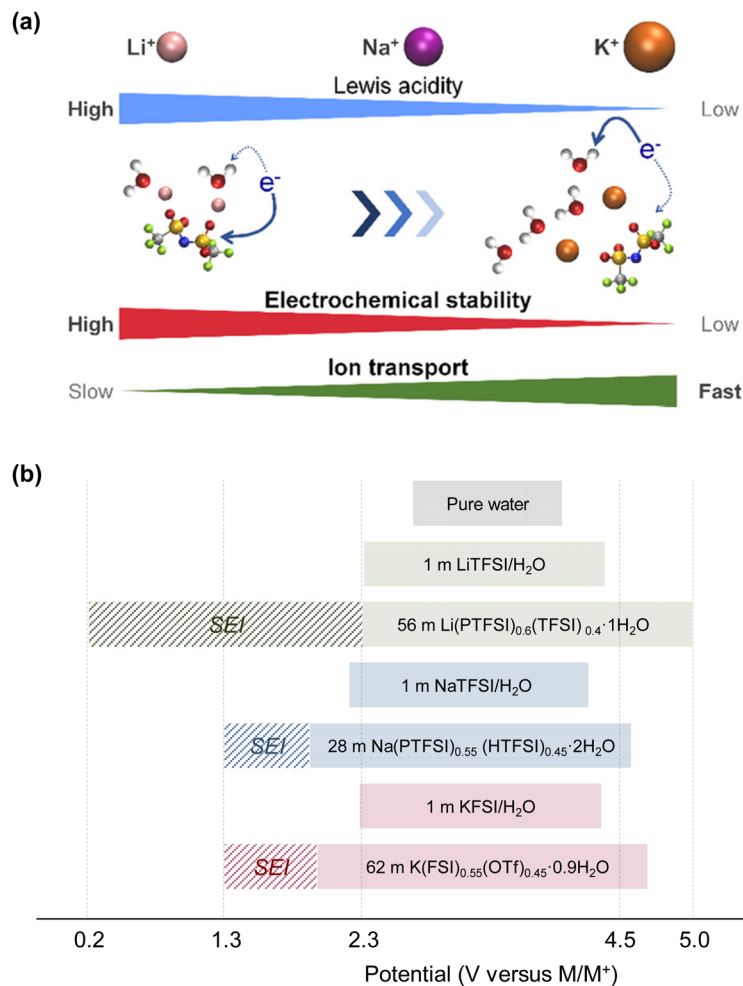
Fig. 15 (a) Carrier ion-dependent electrochemical and physicochemical properties of hydrate melts. 198 Reprinted with permission from ACS Applied Materials & Interfaces. (b) Comparison of aqueous electrolytes based on salt concentration and carrier ion types. The plot was created based on the LSV results obtained using Al and Pt as working electrodes. The areas marked with bold colors and diagonal lines represent the operating potential window of each electrolyte and the kinetic (SEI) contributions within it, respectively. 91,170,185
