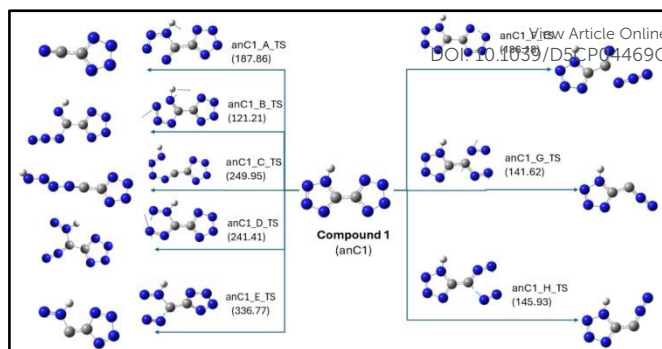
Fig. 11 Transition states obtained for the anionic form of compound 1
