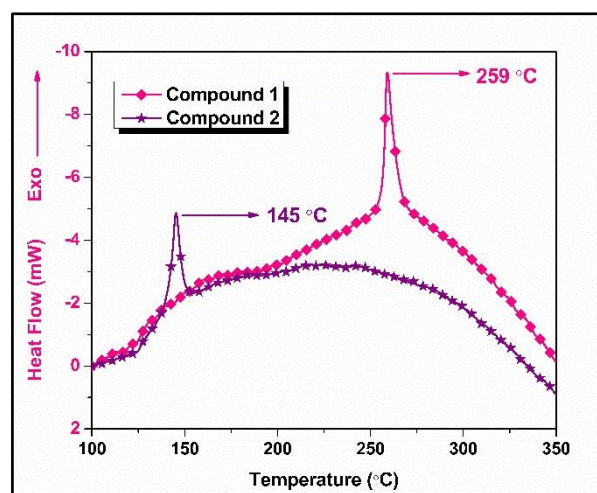
Fig. 4 DTA curves of compounds 1 and 2 at a heating rate of 2.5 °C
