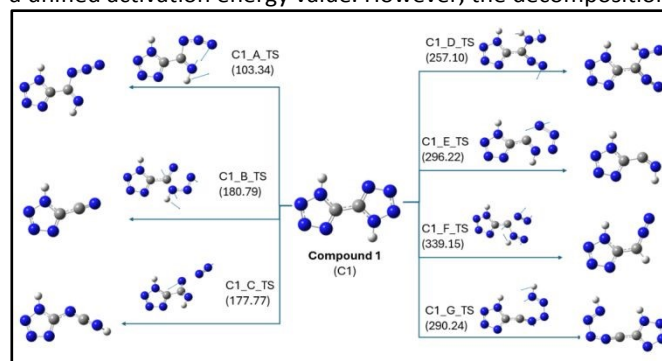
Fig. 7 Transition states for the degradation of compound 1 along with their energies (in kJ/mol)
