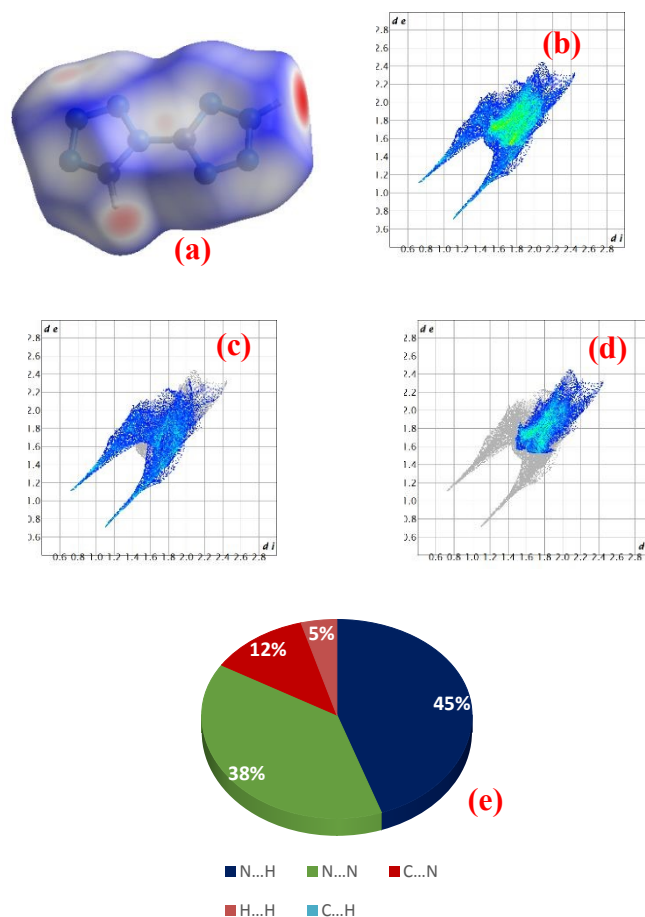
FIG. 17. (a) Hirshfeld surface of compound 2 , (b) the 2D fingerprint plot in the crystal stacking for compound 2 , (c) the contribution of N...H and (d) N...N contacts to the Hirshfeld surface, and (e) pie chart showing % contributions to the Hirshfeld surface from the individual atomic contacts
