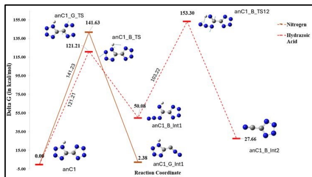
Fig. 12 Degradation pathway for the anionic form of compound 1
