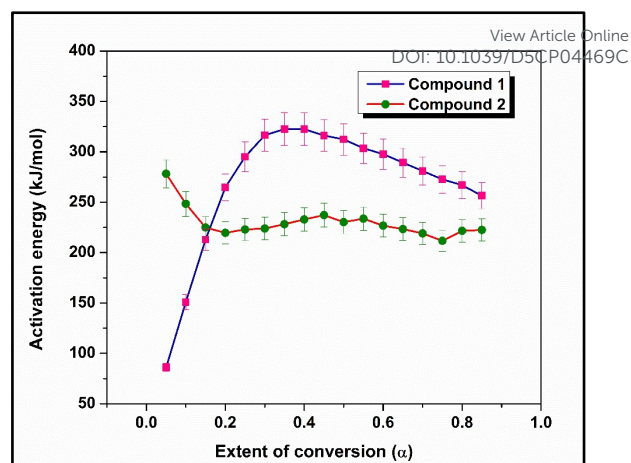
Fig. 6 E_a – \alpha curves of compounds 1 and 2
