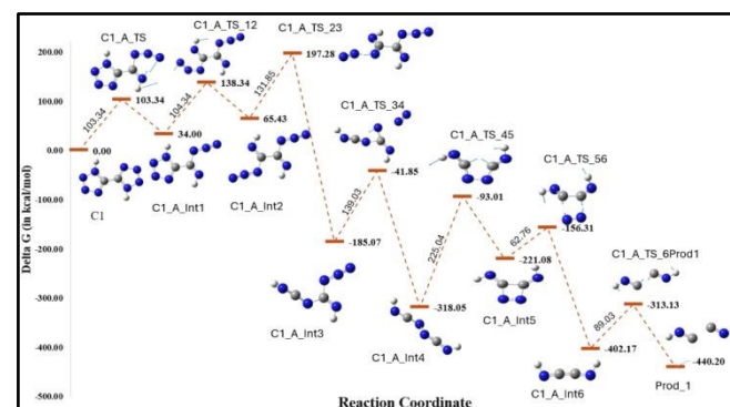
Fig. 8 Unimolecular degradation pathway for compound 1
