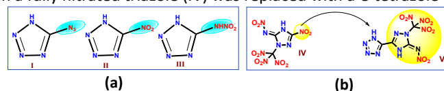
Fig. 1 (a) Sensitive molecules with explosophoric group linked to tetrazole ring (I 8 , II 9 , III 10 ), (b) C-triazole derivatives 13
