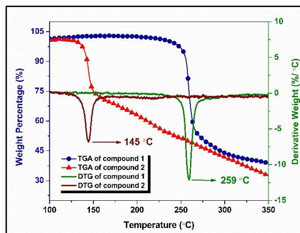
Fig. 3 TGA and DTG curves of compounds 1 and 2 at a heating rate of 2.5 °C/min
