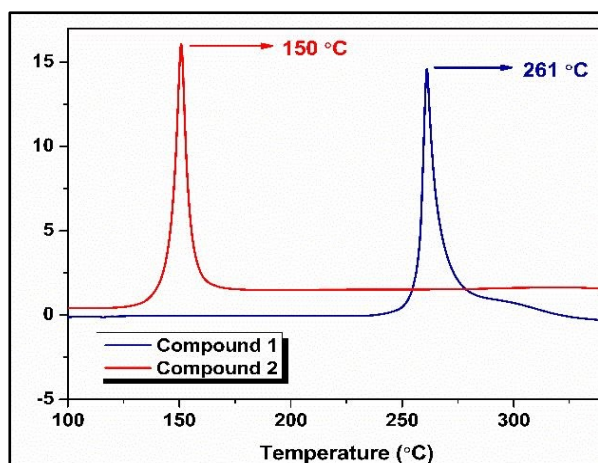
Fig. 5 DSC curve of compounds 1 and 2 at a heating rate of 5 °C/min
