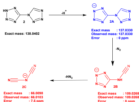
Scheme 1 Possible fragmentation pathway of compound 2
