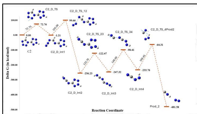
Fig. 10 Unimolecular degradation pathway for compound 2
