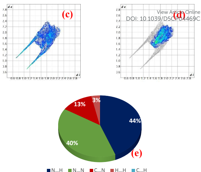
FIG. 16. (a) Hirshfeld surface of compound 1 , (b) the 2D fingerprint plot in the crystal stacking for compound 1 , (c) the contribution of N...H and (d) N...N contacts to the Hirshfeld surface, and (e) pie chart showing % contributions to the Hirshfeld surface from the individual atomic contacts
