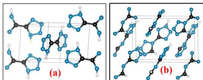
Fig. 15 Crystal structures of compounds 1 31 (a) and 2 20 (b)
