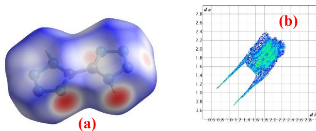
FIG. 17. (a) Hirshfeld surface of compound 2 , (b) the 2D fingerprint plot in the crystal stacking for compound 2 , (c) the contribution of N...H and (d) N...N contacts to the Hirshfeld surface, and (e) pie chart showing % contributions to the Hirshfeld surface from the individual atomic contacts
