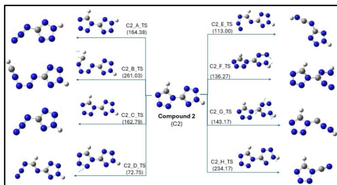
Fig. 9 Transition states for the degradation of compound 2 along with their energies (in kJ/mol)
