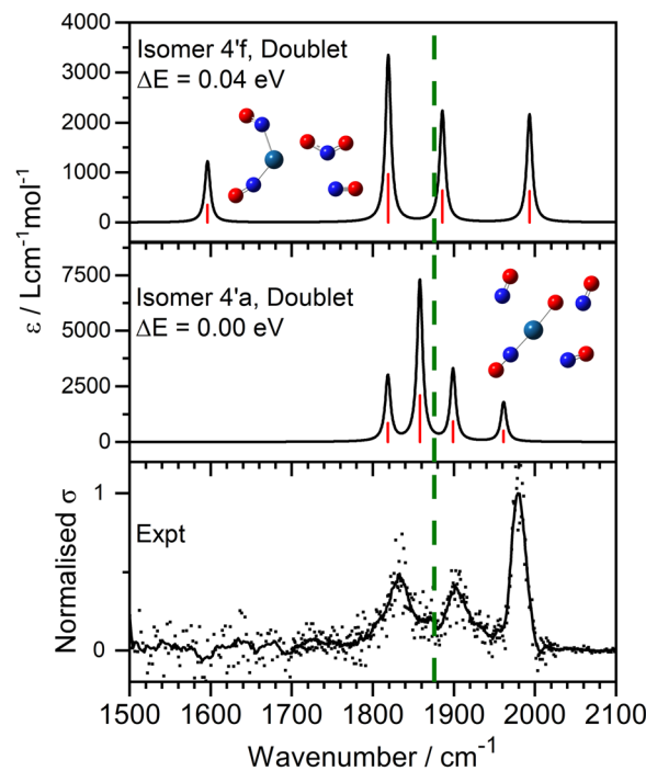
Fig. 6 Experimental IRPD spectra (bottom panel) along with the simulated IR spectra and structures (top panel(s)) for the best-fit low-lying isomers for [\text{PtO}(\text{NO})_4]^+ . The green dashed line indicates the free NO stretch at 1875.84 \text{ cm}^{-1,79,80}
