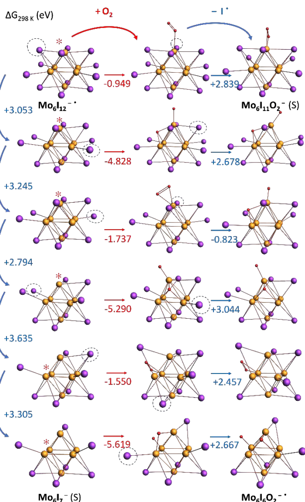
Figure 7. Difference of Gibbs free energy at 298 K of sequential iodine loss and O 2 addition reactions starting from the most stable isomer of (6,12,0)^{1-} . These energies (in eV) correspond to the reaction leading to the most stable possible isomer (S = singlet state; more details in SI). The red star indicates the Mo centre close to which the O 2 molecule was positioned to generate the (6,n,2)^{1-} initial geometry. The dotted circles show which iodine atom was removed to yield the most stable (6,n-1,0)^{1-} and (6,n-1,2)^{1-} isomers. See SI Table S4 for all reaction energy changes.
