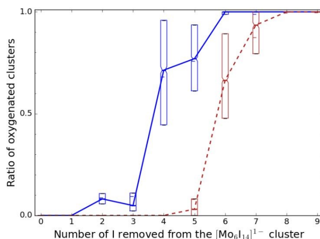
Figure 8. Evolution, as a function of the number of I removed from the precursor, of the complex oxygenation ratio (continuous line) calculated as the sum of all (6,k,2n)^{1-} ion intensities ( n \geq 1 ) normalized by the sum of all (6,k,2n)^{1-} ion intensities ( n \geq 0 ). Dashed red line corresponds to the ratio of multiple oxygenation [(6,k,2n+2)^{1-}] ( n \geq 1 ) normalized by (6,k,2n)^{1-} ( n \geq 0 ). Data is averaged from the 4 experimental fragmentation ranges in the UV and visible ranges.
