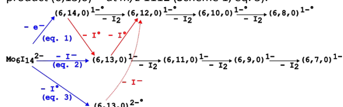
Scheme 1. Three independent photofragments are initially generated by irradiation (blue arrows): loss of an electron (eq. 1), loss of iodide ( \text{I}^- , eq. 2) and loss of iodine ( \text{I}^\bullet , eq. 3). Clusters depleted in iodine ((6,12,0) 1• to (6,7,0) 1• ) are also observed and may arise as secondary fragments from further losses of \text{I}_2 (black arrows) or \text{I}^\bullet (red arrows, attested by CID, see Fig. S1–S2). Loss of \text{I}^\bullet is also observed by CID of (6,13,0)^{2-\bullet} (red dotted arrow, see Fig. S3).
