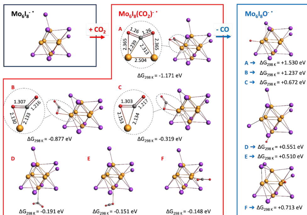
Figure 11. Difference of Gibbs free energy at 298 K for the sequential addition of \text{CO}_2 and loss of CO to the most stable isomer of (6,8,0)^{1-} . All possible coordination de-coordination sites are considered. See SI Table S4 for all reaction energy changes.
