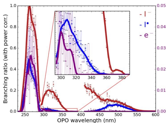
Figure 4. Distribution of the three primary fragments relative intensities as a function of the wavelength. Boxplots represent the 1 st and 3 rd quartiles of the branching ratios corrected for the laser power profile for the loss of \text{I}^- (red) and loss of \text{I}^\bullet (blue) on the left
