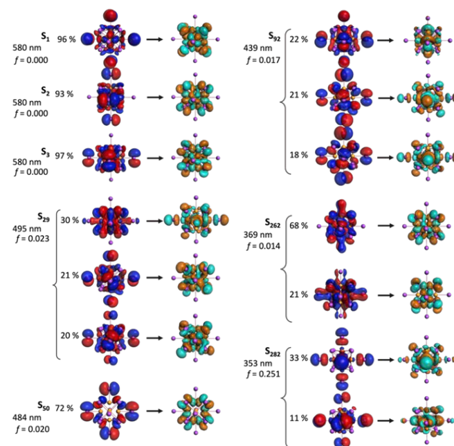
Figure 5. Electron/hole natural transition orbital representations of the three lowest degenerated excited states, and of the excited states of [\text{Mo}_6\text{I}_{14}]^{2-} which oscillator strengths f > 0.007 (only one of the three degenerated states is represented in each case).
