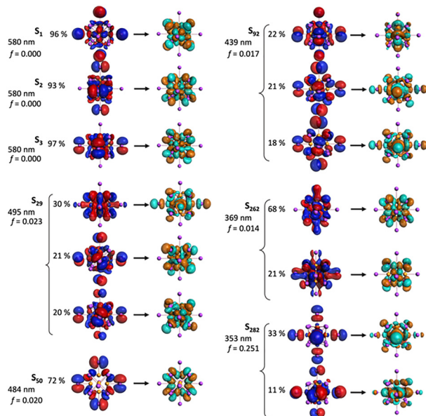
Fig. 5 Electron/hole natural transition orbital representations of the three lowest degenerated excited states, and of the excited states of [\text{Mo}_6\text{I}_{14}]^{2-} with oscillator strengths f > 0.007 (only one of the three degenerated states is represented in each case).
