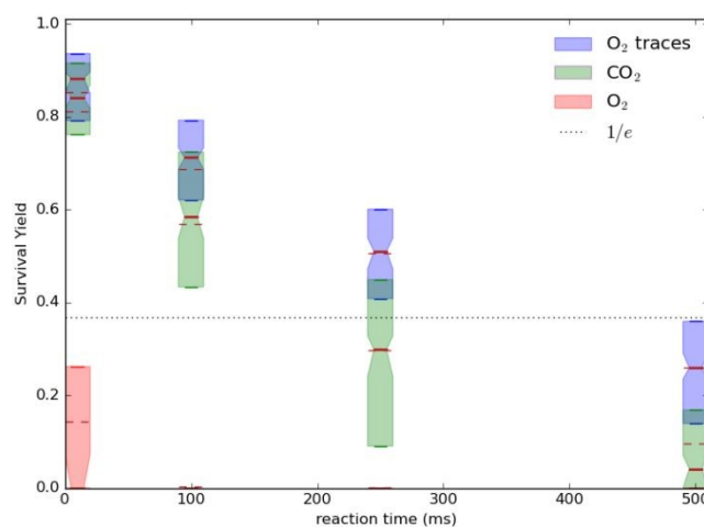
Figure 9. Evolution of the precursor ion [\text{Mo}_6\text{I}_{13}]^{2-} survival yield after variable reaction times in the ion trap filled with various background gas composition: He with unavoidable traces of \text{O}_2 , 0.5 % \text{O}_2 seeded in helium, 0.5% \text{CO}_2 seeded in helium. Boxplots boundaries represent the first and 3 quartiles; thick continuous and thin dashed red lines show the respective positions of the median and the mean for each reaction time dataset. Notches give impressions of the uncertainty windows estimated via a bootstrap approach. The dotted line corresponds to the 1/e level relevant for mono-exponential decays.
