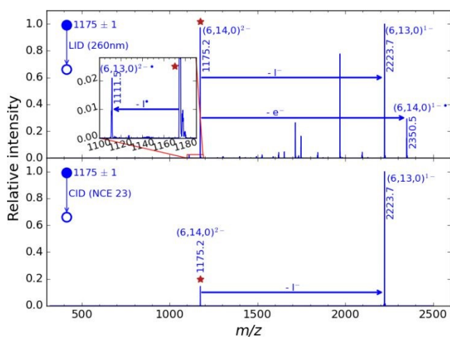
Figure 1. (top) Photo-fragmentation spectrum (LID) at 260 nm and (bottom) collision-induced dissociation (CID) of a single isotopic peak ( m/z 1175.2) of the precursor ion (6,14,0)^{2-} denoted by a star (see the nomenclature section of fragments annotations). Both the oxidized (electron-photo-detached) (6,14,0)^{1-} mono-anion species at m/z 2350.5 and the (6,13,0)^{2-} dianionic species at m/z 1111.5 resulting from the I^{\bullet} photocleavage are photo-specifically formed. Primary fragments are denoted with thick blue arrows. See SI Table S1 for details on assignments.
