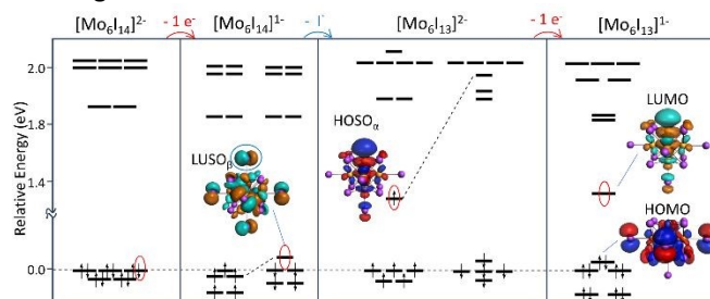
Figure 2. (Spin)orbital molecular energy diagram of [Mo_6I_{14}]^{2-} , [Mo_6I_{14}]^{1-} , [Mo_6I_{13}]^{2-} , and [Mo_6I_{13}]^{1-} . For each system the molecular orbital or spin-orbital \alpha ( HOSO_{\alpha} ) with the same spatial extension and sign as the highest occupied molecular orbitals (HOMO) of the [Mo_6I_{14}]^{2-} , were energetically aligned with it. LUMO = lowest unoccupied molecular orbital. LUSO = lowest unoccupied spin-orbital ( \alpha or \beta ). Isocontours = \pm 0.02 (e.bohr) 3/4 . The plots of all frontier (spin)orbitals are given in Figure S4.
