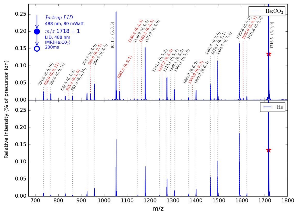
Figure 10. Ion-molecule reactions under irradiation (photo-IMR-MS 2 ) spectra of precursor species (6,9,0)^{1-} . No collisional energy is applied but precursors are irradiated with a CW laser at 488 nm (80 mW) during the whole experiment, from the ion accumulation/injection time, through the 200 ms reaction time with the background gas and up to ion detection. Background gas composition: helium with \text{O}_2 traces (bottom) and He seeded with 0.5% \text{CO}_2 (top). (6,n,2k)^{1-} adducts formed by reaction with \text{O}_2 are marked in black while (6,n,2k+1)^{1-} adducts specifically formed in the presence of \text{CO}_2 are marked in red. See SI Table S2 for details on assignments.
