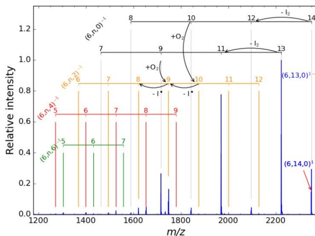
Figure 6. Photo-fragmentation spectrum (LID) at 260 nm of a single isotopic peak ( m/z 1175.2) of the precursor ion (6,14,0)^{2-} denoted by a star (zoom on LID spectrum shown in Figure 1). The focus is made on secondary fragment ion series: (6,n,0)^{1-} iodine-depleted ions (grouped in I_2 loss series), and (6,n,2k)^{1-} reaction products with one, two and three O_2 molecules. Example of -I_2 / +O_2 / -I^* inter-series connectivity is shown with curved black arrows. See SI Table S1 for details on assignments.
