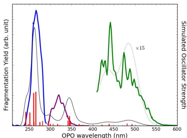
Figure 3. Optical action (fragmentation) spectrum of [\text{Mo}_6\text{I}_{14}]^{2-} in the UV-visible range. The photo-fragmentation was recorded independently for three regions: <290 nm (blue), [290-390] nm (purple) and >410 nm (green). Laser irradiance and alignment conditions vary between regions so that their absolute intensities should not be compared. Thus, experimental data was scaled to ease the comparison with the simulated spectrum. Data was recorded with a 2 nm pitch. Circles on the experimental curves represent the position of the laser alignment for each spectral range. The simulated spectrum (thin black line) is calculated from 0.12 eV gaussian convolution of the oscillator strength for each transition (red bars). A factor \times 15 is applied to simulated data in the visible range (dotted line).
