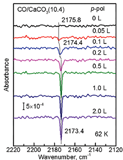
Fig. 11 IRRAS spectra with p -polarized light for \text{CO} adsorbed on the calcite (10.4) surface at 62 K with increasing exposures (0–2 L). Adapted from ref. 34 with permission from Royal Society of Chemistry, copyright 2021.
