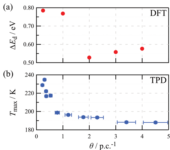
Fig. 4 Comparison between DFT and TPD results. Shown are (a) the desorption energy \Delta E_d estimated by DFT calculations and (b) the peak temperature T_{max} of the \alpha peak from the TPD experiments as functions of water coverage.
