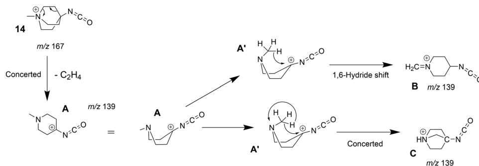
Scheme 5 Fragmentation mechanism of the ethylene-loss observed in the \text{MS}^3 product ion spectrum of the quinuclidinium isocyanate 14 (see Fig. S25, ESI†).
