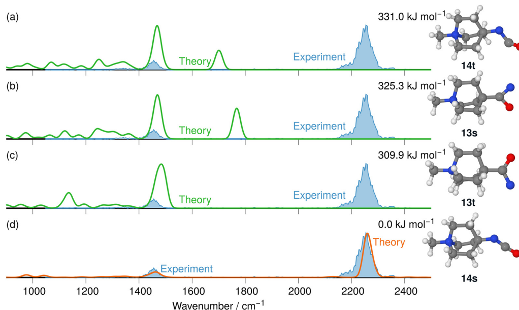
Fig. 7 IR ion spectrum of the \text{N}_2 -loss product ion at m/z 167 of precursor ion 8 (blue shaded trace), compared with the calculated IR spectra of four structural alternatives for the nitrene and the isocyanate ions 13 and 14 : (a) IR spectrum of the triplet isocyanate 14t (harm. frequency calculation, +331.0 \text{kJ mol}^{-1} ); (b) singlet nitrene 13s (harm. frequency calculation, +325.3 \text{kJ mol}^{-1} ); (c) triplet nitrene 13t (harm. frequency calculation, +309.9 \text{kJ mol}^{-1} ); (d) singlet isocyanate 14s (anharm. frequency calculation, 0.0 \text{kJ mol}^{-1} , Table S26, ESI†). All energies were evaluated at the CASPT2//cc-pVTZ level. Scaling of harmonic/anharmonic spectra below 2000 \text{cm}^{-1} : 0.97/0.99. Scaling of harmonic/anharmonic spectra above 2000 \text{cm}^{-1} : 0.95/0.985.
