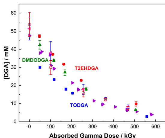
Fig. 5 DGA concentrations as a function of absorbed gamma dose in n -dodecane: TODGA (■), T2EHDGA (●), and DMDODGA (▲) from this work. Previously reported values for: TODGA (▶), 32 TODGA (◀), 12 and T2EHDGA (○) 12 are included for comparison.
