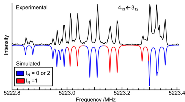
Fig. 5 Experimental and simulated ^{14}\text{N} nuclear quadrupole hyperfine components of the 4_{13} \leftarrow 3_{12} rotational transition. The nuclear quadrupole coupling scheme used is: I_{\text{Ni}} + I_{\text{No}} = I_{\text{N}} ; I_{\text{N}} + J = F . If the two nitrogen nuclei were equivalent, only the blue components with I_{\text{N}} = 0 and 2 would be present in the ground tunnelling state, whereas only the red components with I_{\text{N}} = 1 would be present in the first excited state and would appear in a different frequency region. See text for discussions. The experimental cavity-based FTMW spectrum is a composite of eight measurements centred at 5222.83, 5222.87, 5222.90, 5223.0, 5223.10, 5223.25, 5223.32, and 5223.37 MHz. Each hyperfine component is split into a pair of Doppler components. 53 The component centred at 5223.3 MHz contains a strong blue and a weak red component.
