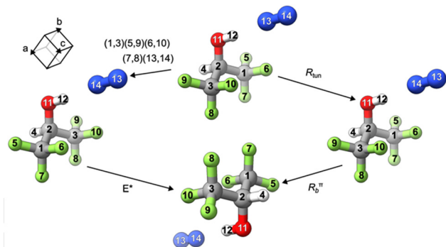
Fig. 4 Visualization of the operation (1,3)(5,9)(6,10)(7,8)(13,14)^* and the associated equivalent rotation R^E_{tun} . Note that the a - and c -axes are in the symmetry plane of the complex, and the b -axis is perpendicular to it.
