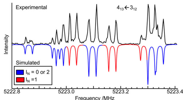
Fig. 5 Experimental and simulated ^{14}\text{N} nuclear quadrupole hyperfine components of the 4_{13}-3_{12} rotational transition. The nuclear quadrupole coupling scheme used is: I_{N1} + I_{N2} = I_N ; I_N + J = F . If the two nitrogen nuclei were equivalent, only the blue components with I_N = 0 and 2 would be present in the ground tunnelling state, whereas only the red components with I_N = 1 would be present in the first excited state and would appear in a different frequency region. See text for discussions. The experimental cavity-based FTMW spectrum is a composite of eight measurements centred at 5222.83, 5222.87, 5222.90, 5223.0, 5223.10, 5223.25, 5223.32, and 5223.37 MHz. Each hyperfine component is split into a pair of Doppler components. 53 The component centred at 5223.3 MHz contains a strong blue and a weak red component.
