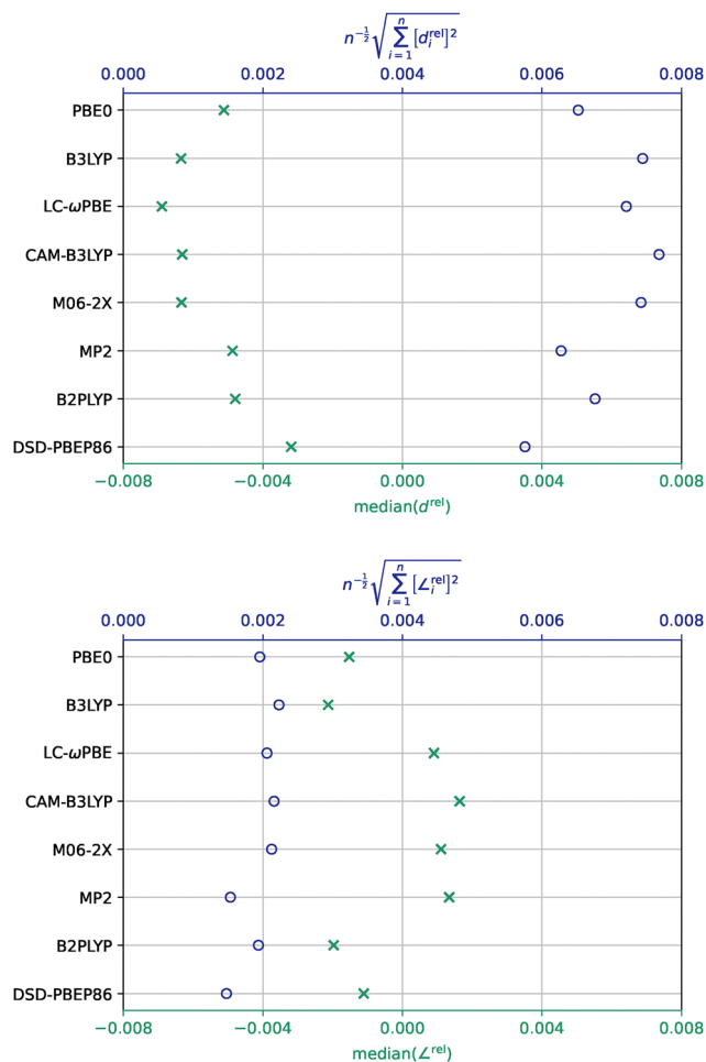
Fig. 8 Comparison of standard and median deviations of bond lengths d^{rel} (above) and angles \angle^{rel} (below) from CCSD(T) for all r_m^{(2)} structures in itaconic anhydride (4 and 4 data points).
