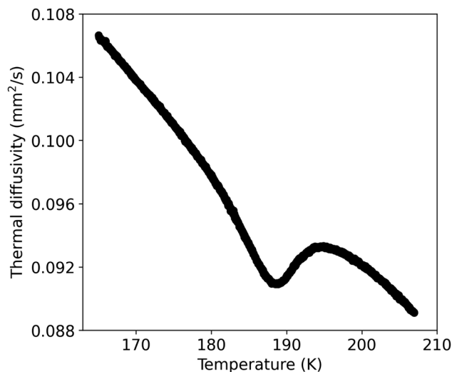
Fig. 4 Temperature dependence of the thermal diffusivity of \text{PIm@}(\text{BC})_2 .
