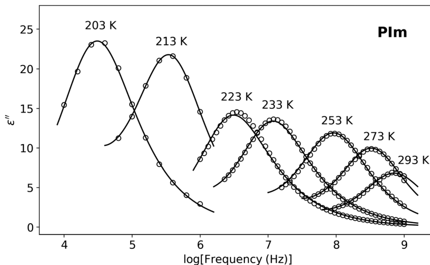
Fig. 2 Dielectric loss spectra of P1m for various temperatures. Lines are fits to the Havriliak–Negami function.
