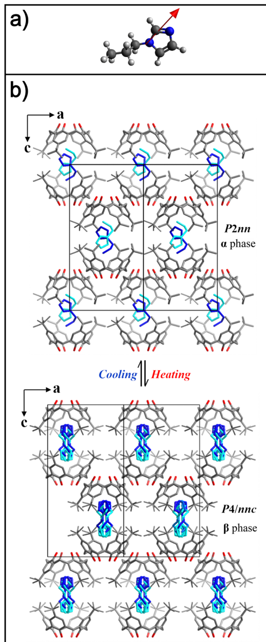
Fig. 1 (a) DFT-optimized geometry and dipole moment of the PIm molecule. (b) Crystal structures of the ferroelectric (a) and paraelectric (b) phases of the PIm@BC 2 clathrate system determined by single-crystal X-ray diffraction. 10
