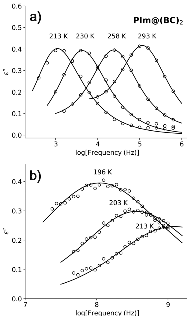
Fig. 5 Dielectric loss spectra of \text{PIm@}(\text{BC})_2 at (a) low frequencies and (b) high frequencies for various temperatures. Lines are fits to the Havriliak–Negami function.
