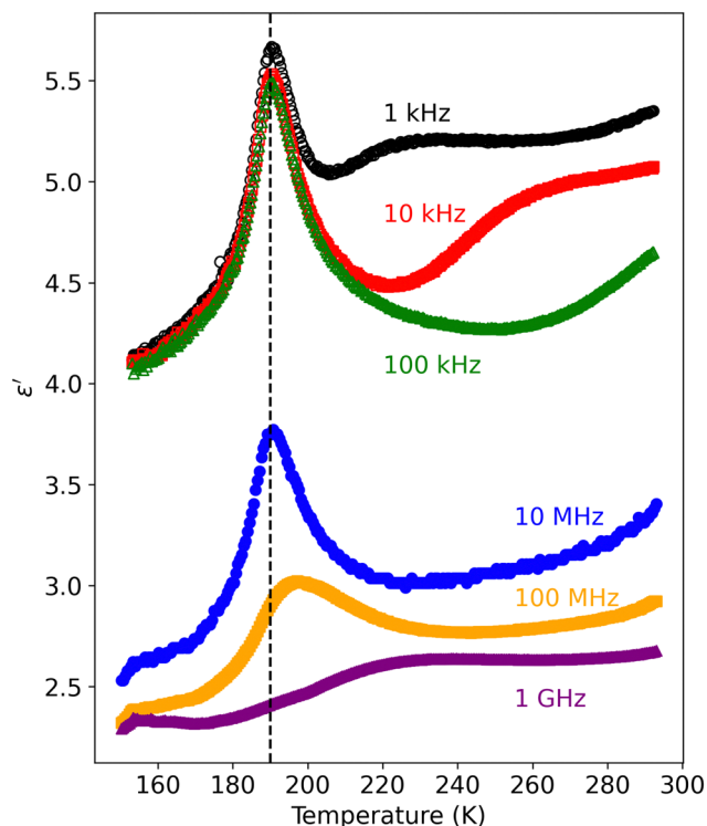
Fig. 3 Temperature dependence of the real part of the complex dielectric permittivity of P1m@BC 2 at selected frequencies. The vertical dashed line corresponds to the ferroelectric phase transition temperature.
