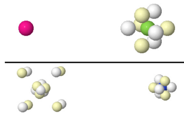
Fig. 6 Born maxima in the LiF (top) and NaCl (bottom) molecules. Different spin electrons are pictured as white/yellow spheres. A pair of spin-coupled electrons lying at each nucleus is not shown.
