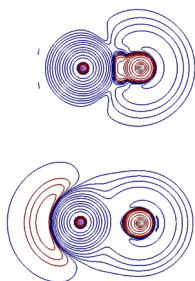
Fig. 5 Isocontours (blue, positive; red, negative) of \nabla^2\rho for the aug-cc-pVDZ/FCI 1^1\Sigma (top) and 2^1\Sigma (bottom) states of LiH at R = 2.0 \text{ \AA} .
