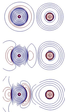
Fig. 4 Isocontours (blue, positive; red, negative) of \nabla^2\rho for the aug-cc-pVDZ/FCI 1^1\Sigma (top), 2^1\Sigma (middle), and 3^1\Sigma (bottom) states of LiH at R = 4.0 \text{ \AA} .
