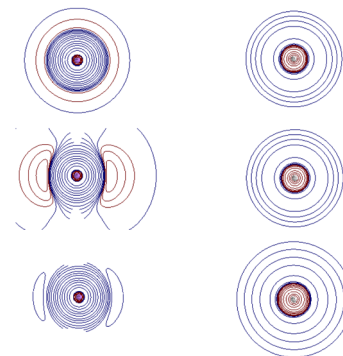
Fig. 3 Isocontours (blue, positive; red, negative) of \nabla^2\rho for the aug-cc-pVDZ/FCI 1^1\Sigma (top), 2^1\Sigma (middle), and 3^1\Sigma (bottom) states of LiH at R = 8.0 \text{ \AA} .
