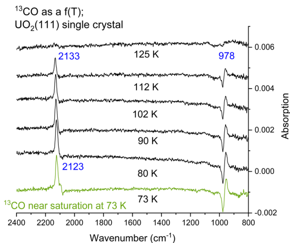
Fig. 4 Difference IRRAS spectra collected after the surface has been exposed to 0.2 L of CO (near saturation) at 73 K. This is followed by flashing the crystal at a rate of 0.1–0.2 \text{K s}^{-1} to the indicated temperatures then cooled back to 73 K for further spectral collection.
