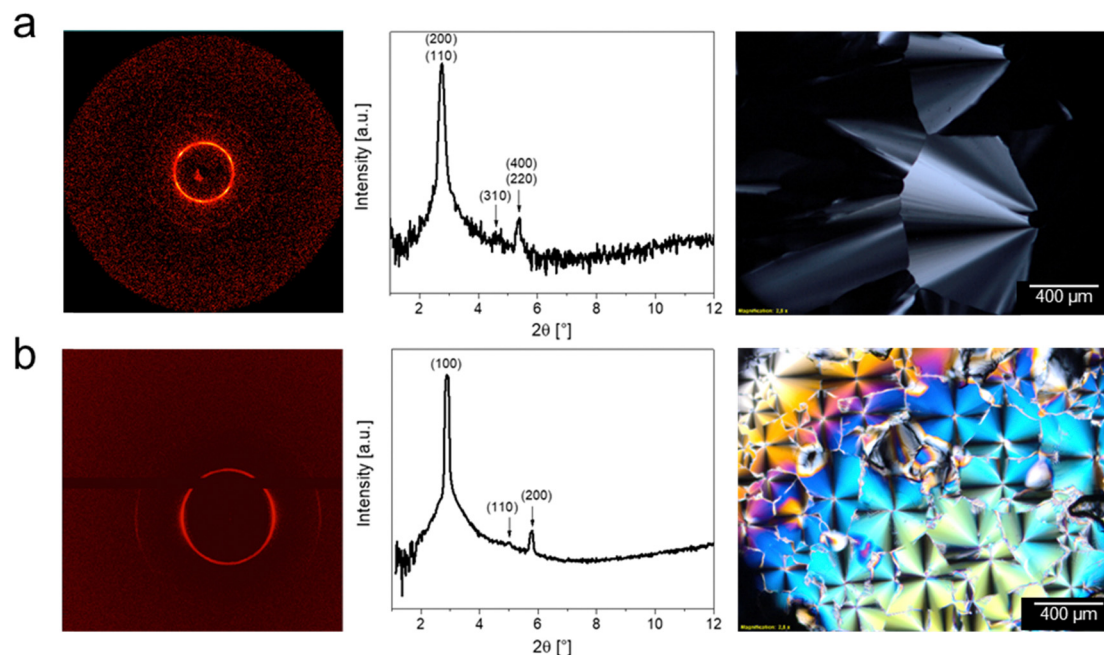
Fig. 7 Comparison of 2D diffraction patterns, diffractograms and POM images of C_{12} based ILCs (a) DmC_{12}S HSO_4 at 25\text{ }^\circ\text{C} , and (b) DmC_{12}S MeSO_3 at 20\text{ }^\circ\text{C} .
