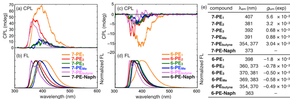
Fig. 3 (a) CPL spectra of 7-PE n . Conditions: 1.0 \times 10^{-5} M in \text{CHCl}_3 , 25 °C. \lambda_{ex} = 280 nm ( 7-PE 1 , 7-PE 2 , 7-PE 3 , 7-PE Me ), 278 nm ( 7-PE butyne ). (b) FL spectra of 7-PE n and 7-PE-Naph . Conditions: 1.0 \times 10^{-5} M in \text{CHCl}_3 , 25 °C. \lambda_{ex} = 278.5 nm ( 7-PE 1 ), 278 nm ( 7-PE 2 ), 279 nm ( 7-PE 3 , 7-PE Me ), 278.5 nm ( 7-PE butyne ), 278 nm ( 7-PE-Naph ). (c) CPL spectra of 6-PE n . Conditions: 1.0 \times 10^{-5} M in \text{CHCl}_3 , 25 °C. \lambda_{ex} = 274 nm ( 6-PE 1 , 6-PE 2 ), 277 nm ( 6-PE 3 ), 286 nm ( 6-PE Me ), 282 nm ( 6-PE butyne ). (d) FL spectra of 6-PE n and 6-PE-Naph . Conditions: 1.0 \times 10^{-5} M in \text{CHCl}_3 , 25 °C. \lambda_{ex} = 284 nm ( 6-PE 1 , 6-PE 2 ), 286.5 nm ( 6-PE 3 ), 276 nm ( 6-PE Me ), 282.5 nm ( 6-PE butyne ), 279 nm ( 6-PE-Naph ). (e) Summary of the photophysical properties of ( S )- 7-PE n , 7-PE-Naph , ( S )- 6-PE n , and 6-PE-Naph .
