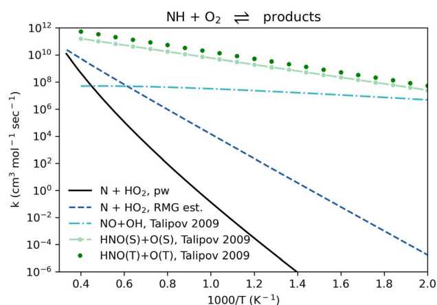
Fig. 2 Comparison of rate coefficients for \text{NH} + \text{O}_2 giving \text{N} + \text{HO}_2 (reaction R1, given in reverse in Table 1) computed here (pw) and compared to RMG's estimate, and giving \text{NO} + \text{OH} and \text{HNO} + \text{O} as recommended by Talipov et al. 64
