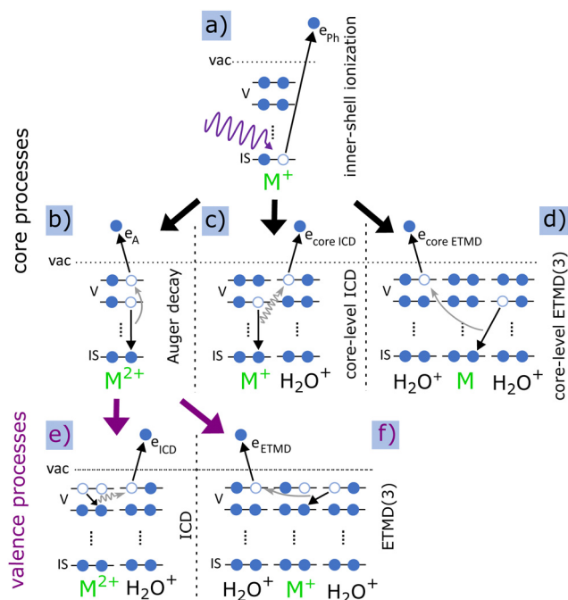
Fig. 1 Schemed local and intermolecular processes after inner-shell photoionisation of pyrimidine (M) embedded in a water cluster, grouped in mechanisms involving the core [(a)–(d)] or valence states [(e) and (f)]. Process (a) is the inner-shell (IS) photoionisation of a molecule M emitting a photoelectron e_{\text{ph}} . Panel (b) displays the subsequent Auger decay where a valence (V) electron fills the core vacancy and another valence electron from the same molecule is emitted (Auger electron e_{\text{A}} ). Process (c) shows the core-level ICD, transferring the released energy to a neighbouring water molecule and ionising a valence electron ( e_{\text{core ICD}} ). Process (d) sketches core-level ETMD(3). Here, a valence electron from neighbouring water fills the inner-shell vacancy of the initially ionised molecule and a valence electron ( e_{\text{core ETMD}} ) from another water is released. ICD and ETMD can additionally happen after a preceding Auger decay [processes (e) and (f)].
