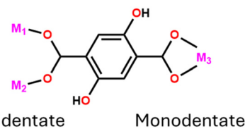
Fig. 4 Scheme of the bidentate and monodentate coordination modes of the \text{DOBDC} linker.
