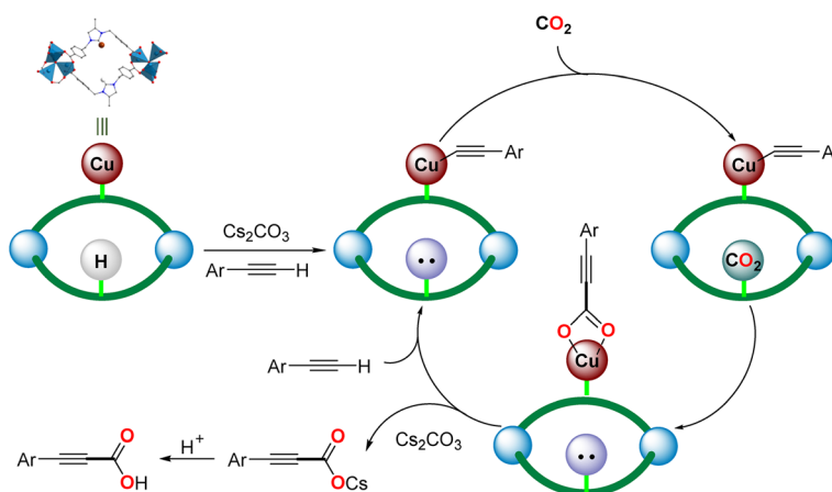
Scheme 2 Possible mechanism of the carboxylation of terminal alkynes with CO 2 .
