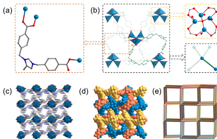
Fig. 1 (a) Coordination mode of the L^- ligand; (b) [\text{Zn}_4(\mu_4\text{-O})(\text{COO})_4] secondary building units connected by L^- ligands; (c) single 3D framework; (d) 3-fold interpenetrated network; and (e) illustration of the 3D topology of the Zn-MOF.
