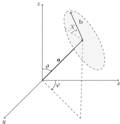
Fig. 2 The angular notation systems \theta , \phi , and \chi used to define the spatial shear modulus, where \mathbf{a} is perpendicular to the shear plane (highlighted in gray ellipse), while \mathbf{b} indicates the direction in which the strain is measured.
