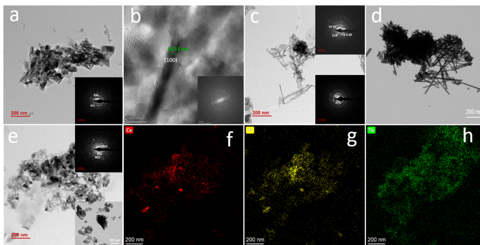
Fig. 3 TEM micrographs of Ap blank (a), Ap-Eu (c and d) and Ap-Tb (e) particles prepared at 200 °C in presence of 10 mM of lanthanide. Insets show the indexed SAED patterns corresponding to Ap (a), small particles of whitlockite and long apatite-Eu crystals (c), and apatite-Tb nanoparticles (e). HR-TEM image of (a) Ap-blank crystals displaying the lattice fringes corresponding to d -spacing of the (100) plane (b). Inset shows the corresponding FFT images displaying the (100) plane. EDX element mapping analysis of Ca (f), P (g) and Tb (h) of the sample shown in micrograph (e).
