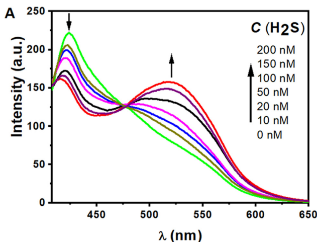
Fig. S12 (A) Fluorescence spectra of CD-based sensor (concentration: 0.15 \text{ mg mL}^{-1} , the amount of probe conjugated onto CDs: 4.48 \text{ mg g}^{-1} ) in the presence of different amounts of \text{H}_2\text{S} in HEPES buffered (pH 7.4) water-ethanol (3 : 1, v/v).
