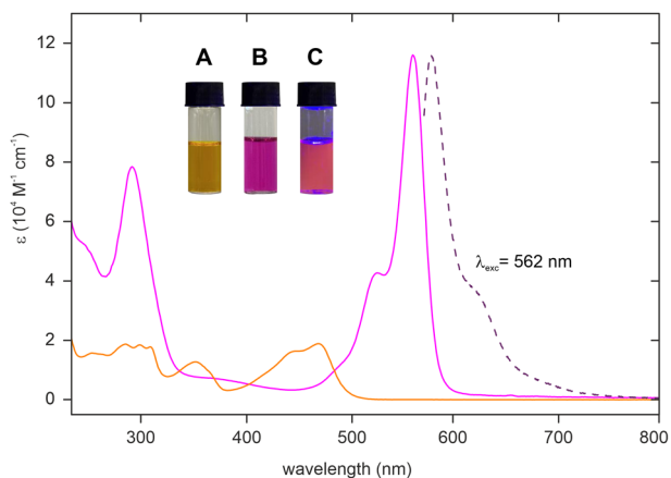
Fig. 3 UV-vis absorption spectra of 3-Zn (orange solid line) and 5-Zn (violet solid line) in \text{CH}_3\text{OH} at 298 K. The dotted line shows the fluorescence spectrum of 5-Zn in \text{CH}_3\text{OH} recorded upon excitation at 562 nm at 298 K. The inset shows the colour of methanolic solutions of (A) 3-Zn , (B) 5-Zn , and (C) 5-Zn under UV light (365 nm).
