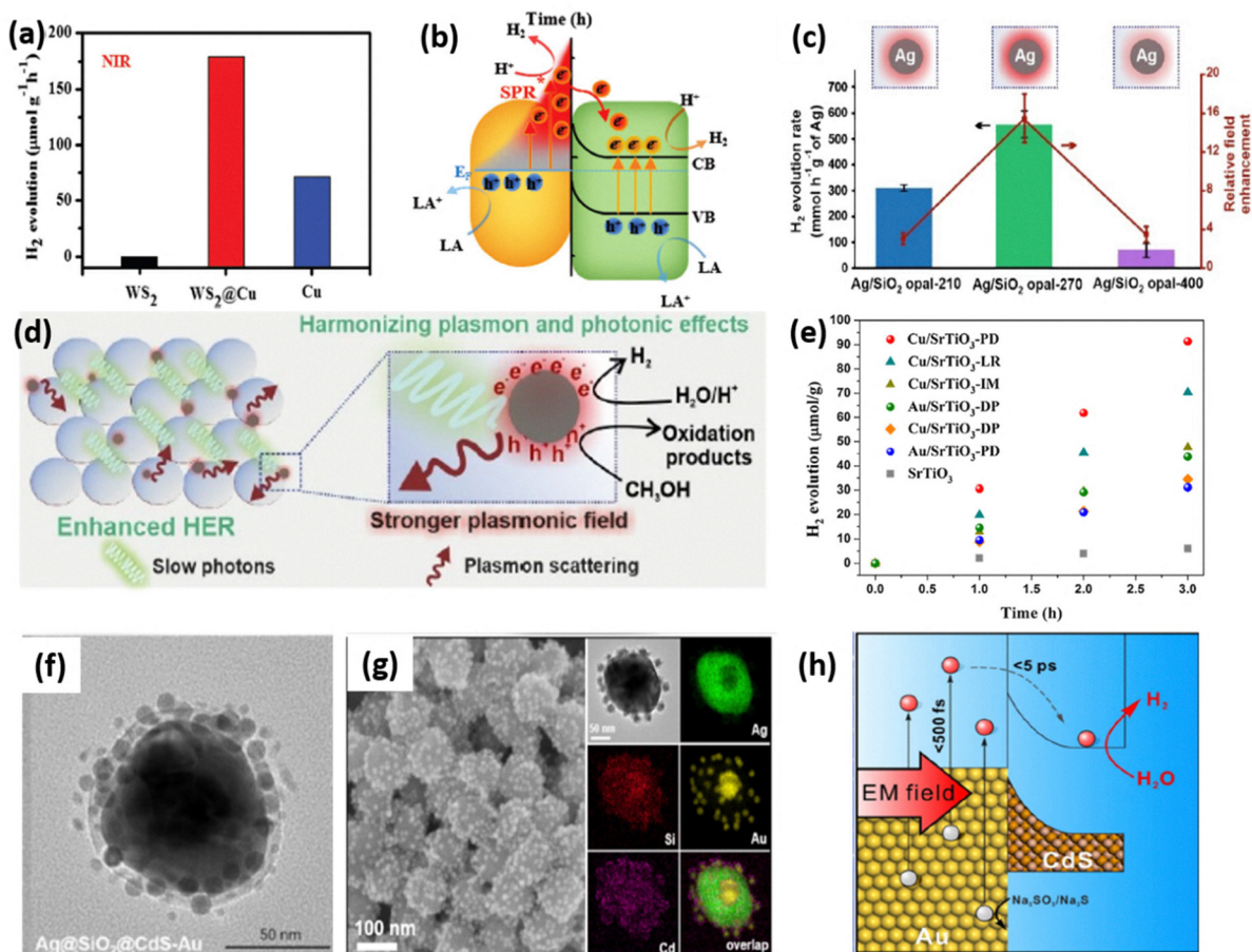
Fig. 4 (a) Photocatalytic \text{H}_2 evolution on photocatalysts upon irradiation of > 750 nm NIR light. (b) Proposed schematic representation of photoinduced charge migration in \text{WS}_2@Cu for photocatalytic \text{H}_2 evolution in the presence of sacrificial agent LA. Reproduced with permission. 56 Copyright 2018, Wiley. (c) \text{H}_2 evolution and associated field enhancement across diverse plasmonic photonic crystals shown, with the inset displaying electromagnetic field strengths for different plasmonic photocatalysts, in agreement with earlier SERS analyses. (d) The superior light absorption of Ag/SiO_2 opal-270 for improved \text{H}_2 evolution. Reproduced with permission. 57 Copyright 2024, Wiley. (e) \text{H}_2 evolution as a function of irradiation time under visible light ( \lambda > 400 nm) for 0.5 wt% Cu/SrTiO_3 and Au/SrTiO_3 . Reproduced with permission. 58 Copyright 2019, Elsevier. (f) HRTEM image of Ag@SiO_2@CdS-Au . Reproduced with permission. 59 Copyright 2020, American Chemical Society. (g) SEM image of Ag SHIN-Au@CdS nanoparticles. The inset illustrates a TEM image and the associated EDS mapping analysis of an individual Ag SHIN-Au@CdS nanoparticle. (h) Schematic illustration of the mechanism for enhancement in \text{H}_2 evolution over Ag SHIN-Au@CdS dual antennas. Reproduced with permission. 60 Copyright 2021, American Chemical Society.
