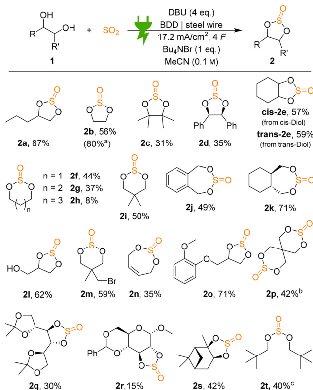
Scheme 2 Scope of sulfites. Conditions: diol 1 (500 \mu\text{mol} , 1 eq., 0.1 M), \text{SO}_2 (5 eq.), DBU (4 eq.), \text{Bu}_4\text{NBr} (1 eq.), MeCN (5 mL), BDD|stainless steel wire, 17.2 \text{mA cm}^{-2} , 4 F, rt. a qNMR yield. b 10 eq. of \text{SO}_2 , 8 eq. of DBU, 2 eq. of \text{Bu}_4\text{NBr} and 8 F. c Neopentanol (600 \mu\text{mol} , 1 eq., 0.1 M), BDD|stainless steel.
