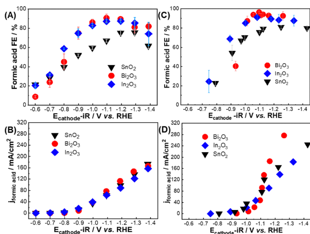
Fig. 1 Formic acid FE and partial current densities as function of iR -corrected cathode potential ( E_{\text{cathode}}-iR ) for \text{Bi}_2\text{O}_3 , \text{In}_2\text{O}_3 , and \text{SnO}_2 in (A, B) aqueous H-cell and (C, D) GDE half-cell configurations. Note that same Y-axis and X-axis scales were plotted for (B) and (D) panels to clearly demonstrate the difference between aqueous H-cell and GDE half-cell current densities over a similar potential range. GDE half-cell results over a larger potential range are shown in Fig. S4 (ESI † ).
