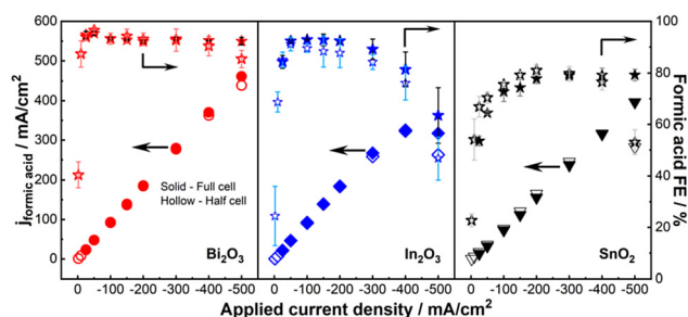
Fig. 2 Comparison of FA partial current densities and \text{FE}_{\text{FA}} for all three catalysts as a function of applied current density in half-cell (hollow) and full cell (solid).
