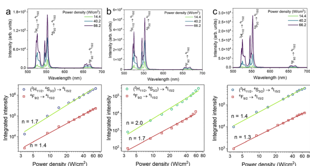
Fig. 4 Upconversion intensity dependence on excitation power density (top panel) to estimate the number of photons involved in the process using the intensity power law (bottom panel). (a) 15% \text{Er}^{3+} , (b) 18% \text{Er}^{3+} and (c) 20% \text{Er}^{3+} .
