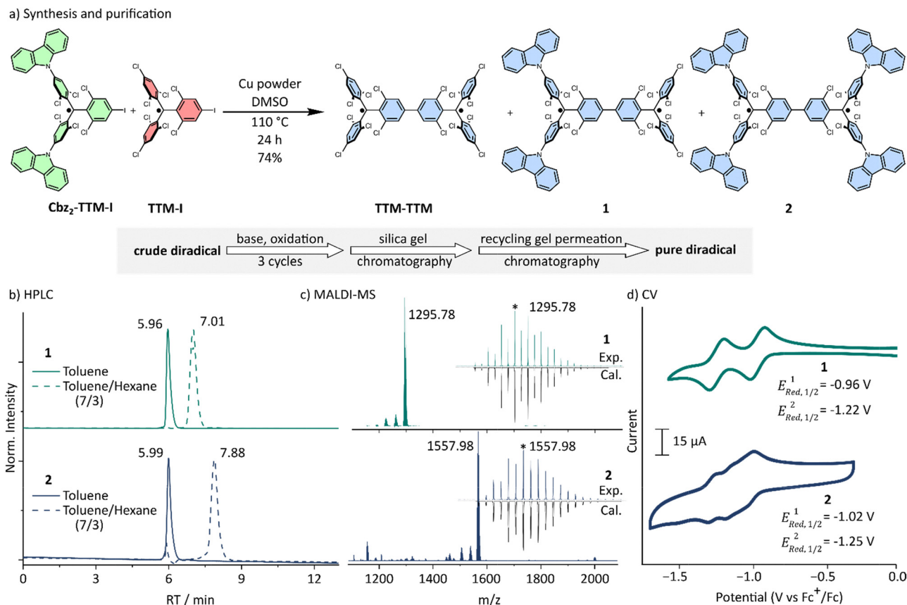
Fig. 2 (a) Statistical Ullmann synthesis of Chichibabin diradicaloids TTM-TTM , 1 , 2 and flow-chart of purification method. (b) Representative HPLC chromatograms (Buckyprep M, 0.5 \text{ mL min}^{-1} ). (c) High-resolution mass spectrometry (HR-MS, MALDI, positive mode) including isotopic patterns. (d) Cyclic voltammograms (CV) at a scan rate of 100 \text{ mV s}^{-1} (glassy carbon (working), Pt wire (counter) and \text{Ag}/\text{Ag}^+ (reference) electrodes, 0.1 \text{ M } ^n\text{Bu}_4\text{NPF}_6 in anhydrous \text{CH}_2\text{Cl}_2 ).
