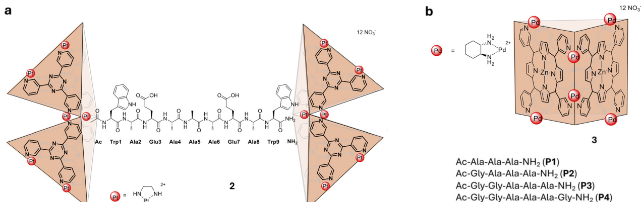
Fig. 2 (a) The 2 : 1 MOC : peptide complex formed with MOC 2 , a Pt 6 L 4 bowl and peptides up to nine amino acids in length; (b) the zinc porphyrin MOC 3 reported to bind short peptides P1 – P4 inducing defined peptide conformations.
