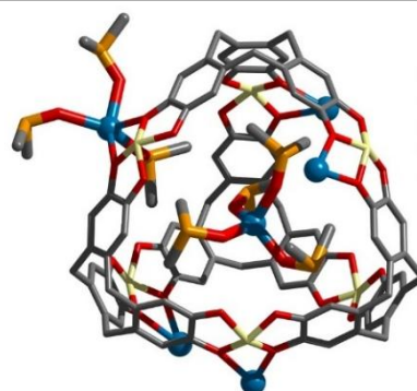
Fig. 3 X-ray structure of H . For the sake of clarity, hydrogen atoms, the n -octyl chains at Si, some of the coordinating DMSO molecules and the second cage are omitted.
