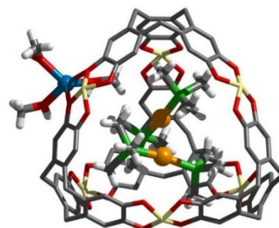
Fig. 5 X-ray crystal structure of GG@H . For the sake of clarity, hydrogen atoms of H , the n -octyl chains at Si and three \text{Na}(\text{MeOH})_3^+ are omitted.
