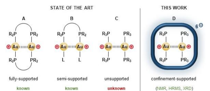
Fig. 1 Aurophilic interactions in gold(I) phosphine complexes.
