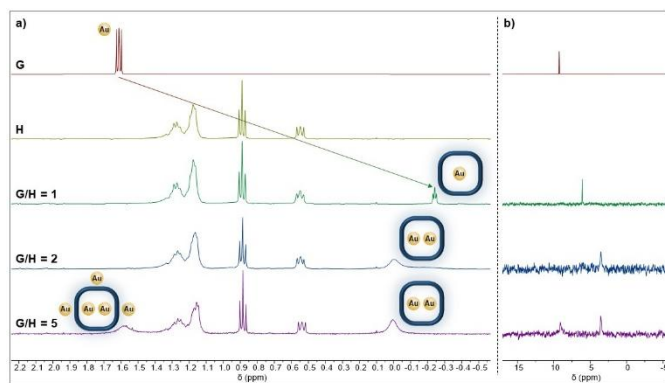
Fig. 5 X-ray crystal structure of GG@H . For the sake of clarity, hydrogen atoms of H , the n -octyl chains at Si and three \text{Na}(\text{MeOH})_3^+ are omitted.
