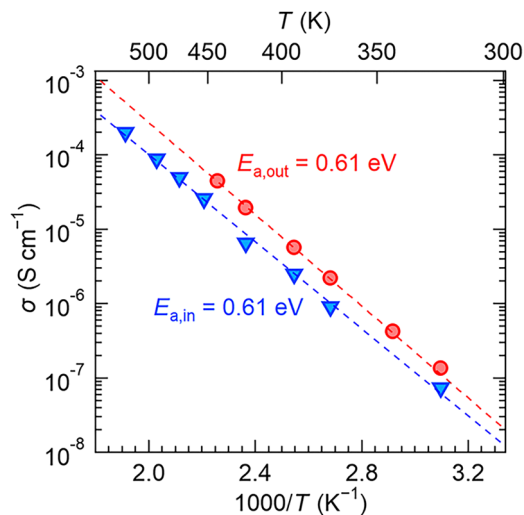
Fig. 5 In-plane (blue) and out-of-plane (red) F-ion conductivity of the \text{Sr}_{0.5}\text{Ce}_{0.5}\text{F}_{2.5} film obtained at T_f = 500 °C as a function of temperature. The dashed line represents the linear fit of the measurements.
