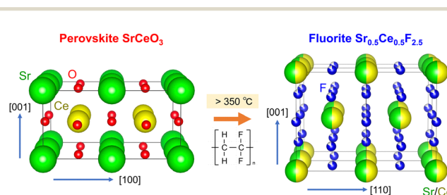
Fig. 4 Schematic of the change in crystal structure of the SrCeO 3 film with polyvinylidene fluoride-mediated fluorination.
