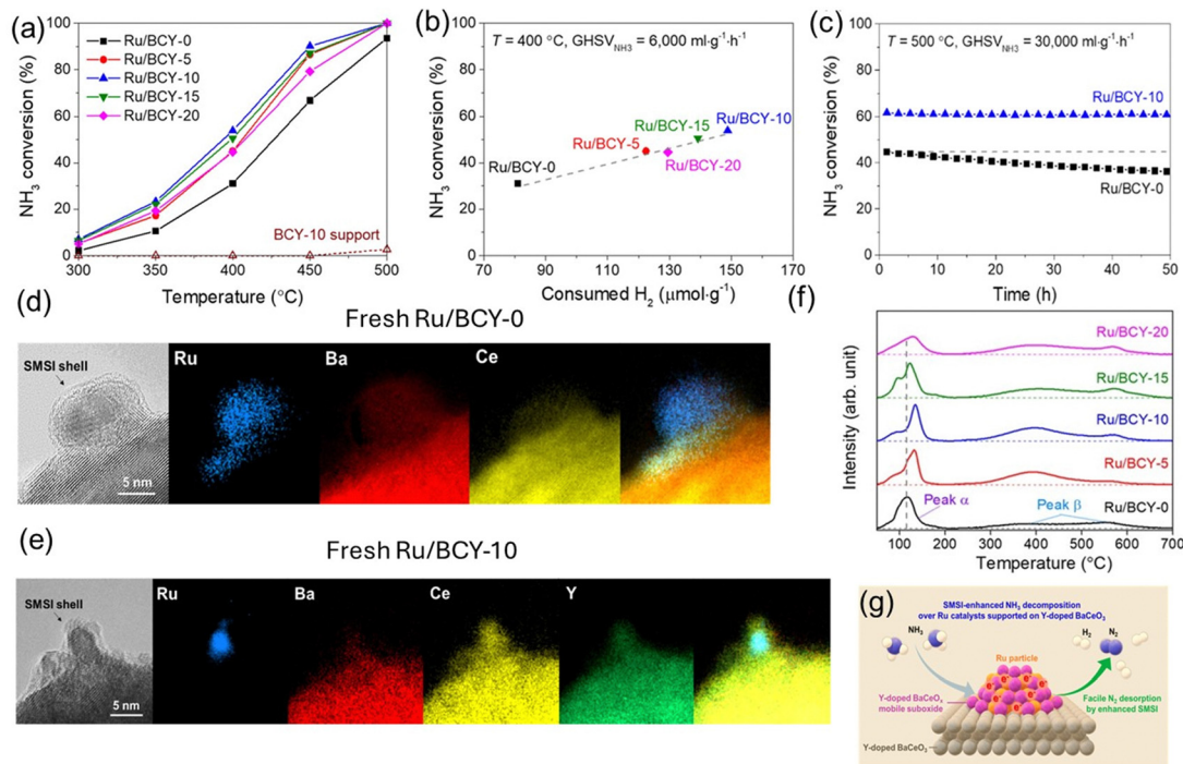
Fig. 6 (a) NH 3 conversion of the Ru/BCY- x catalysts and BCY-10 support as a function of temperature (300–500 °C). (b) NH 3 conversion as a function of H 2 consumption for O 2 removal during H 2 -TPR at 400 °C, GHSV NH 3 = 6000 mL g cat -1 h -1 , and 100 mg of catalyst, (c) long-term stability of the Ru/BCY-0 and Ru/BCY-10 catalysts for a reaction period of 50 h (d) and (e) HR-TEM and EELS mapping images of the prerduced Ru/BCY-0 and Ru/BCY-10 catalysts. NH 3 conversion of the Ru/BCY- x catalysts and BCY-10 support as a function of temperature. (f) H 2 -TPR profiles of the as-prepared Ru/BCY- x catalysts (g) schematic representation of SMSI on NH 3 conversion. (Reproduced with the permission from. 116 Copyright (2022) American Chemical Society).
