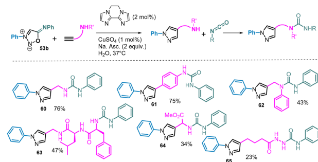
Scheme 22 Cascade reaction.
