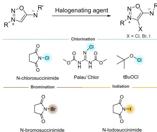
Scheme 8 Halogenation of 4-C position of SI .
