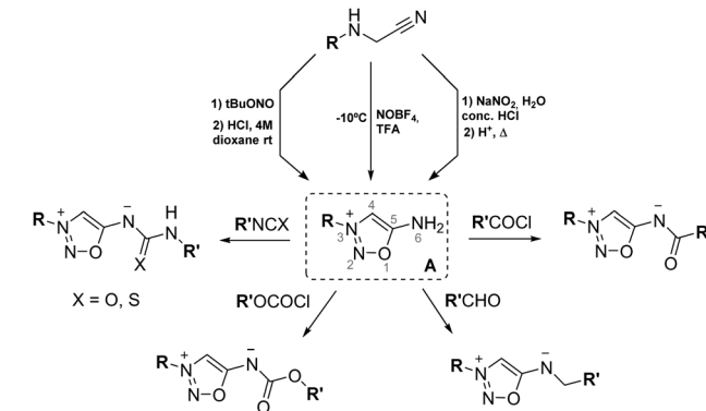
Scheme 2 General synthetic routes to sydnonimines.
