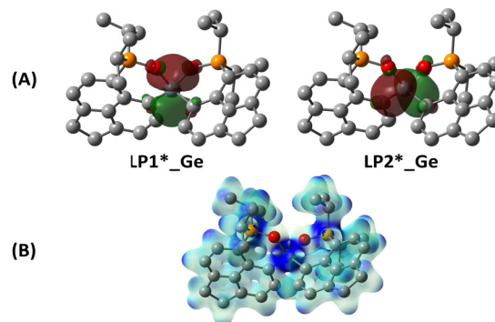
Fig. 3 (A) Natural bond orbitals localized on the Ge center; (B) electrostatic potential map with the range of 0.05 (red)–0.40 (blue).
